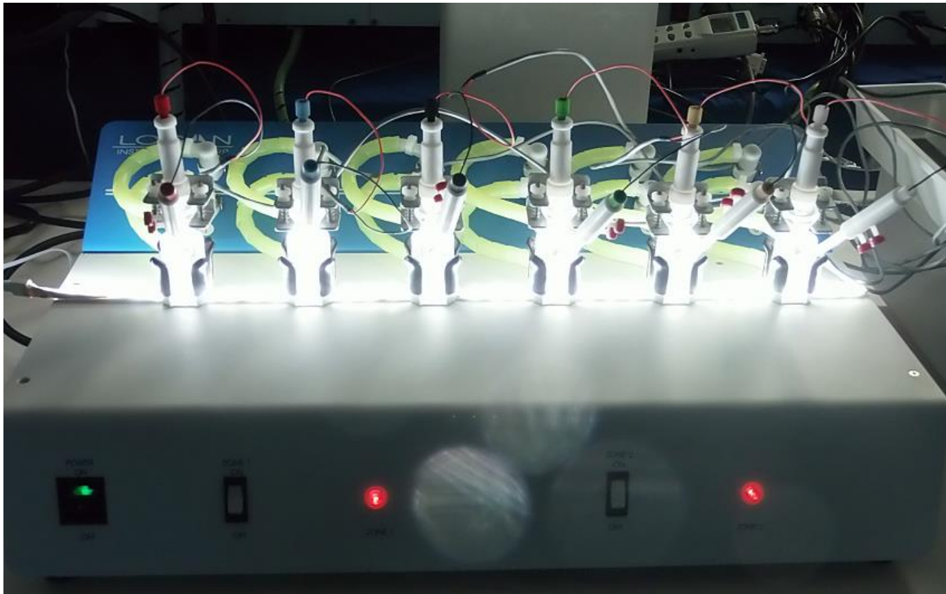
Vertical Diffusion Cell electrode system
