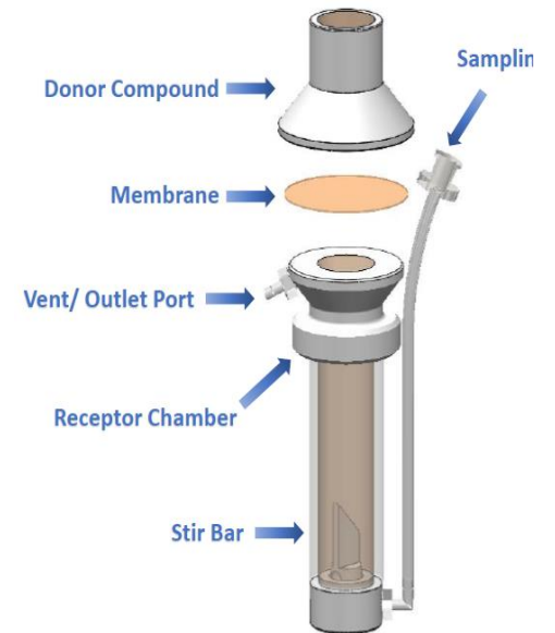
Bubble Free Dry Heat Cell
