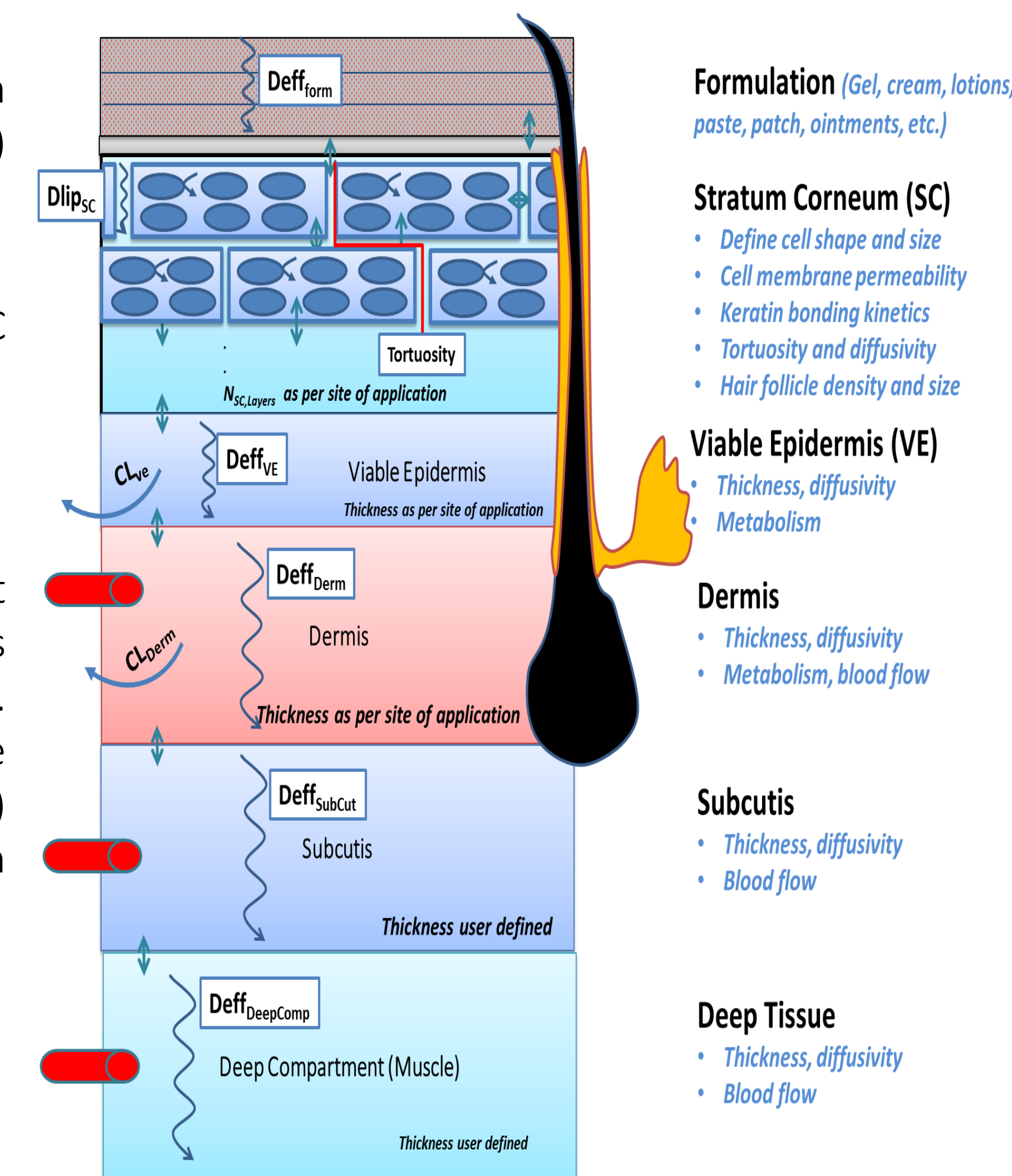
Figure 1. MPML MechDerma Model with a brick (cuboid corneocytes)-and-mortar (intercellular lipids) structure
