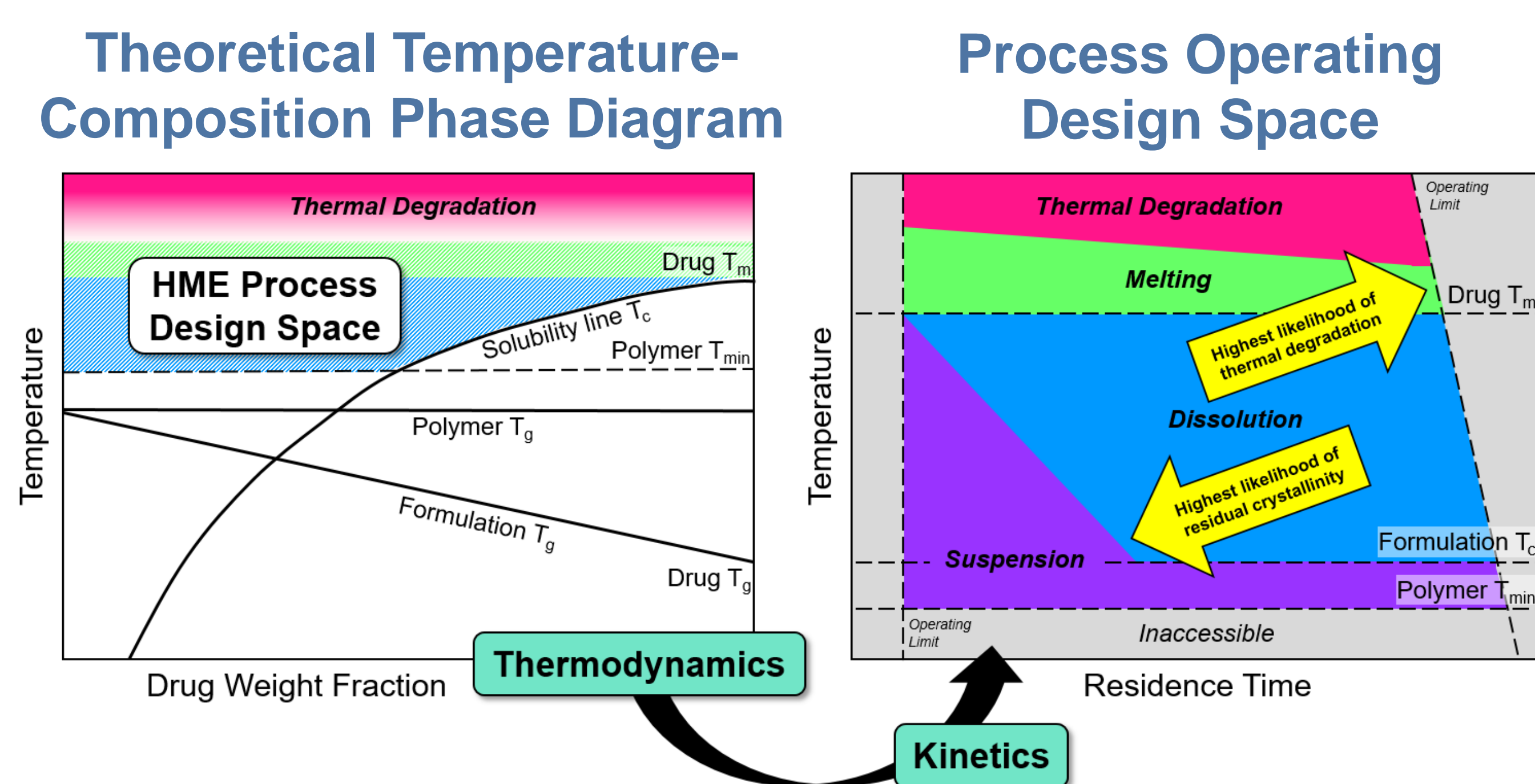
Figure 1. The temperature-composition phase diagram for a drug-polymer system can be used to guide processing temperature selection. By incorporating kinetic criteria, a process operating design space diagram can be constructed.
