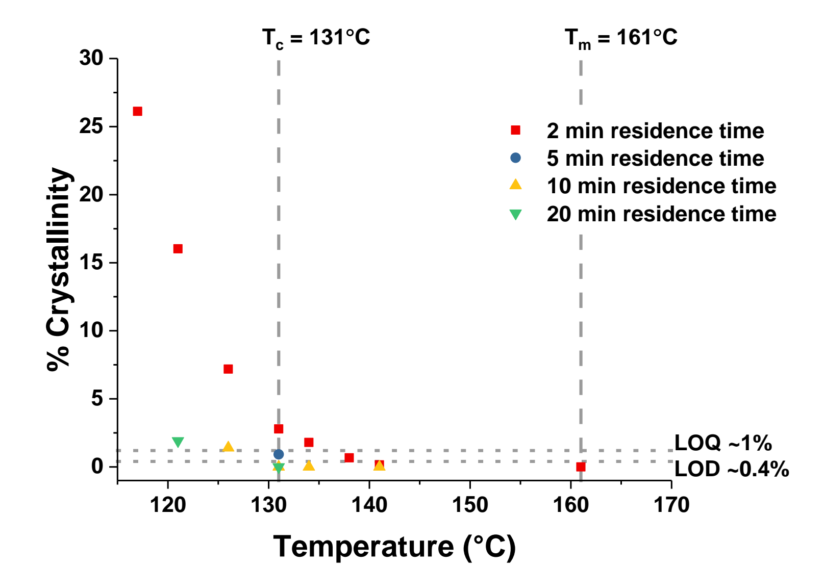
Figure 4. Quantification of crystalline content of 1:1 indomethacin:PVPVA ASDs by XRPD as a function of product melt temperature.
