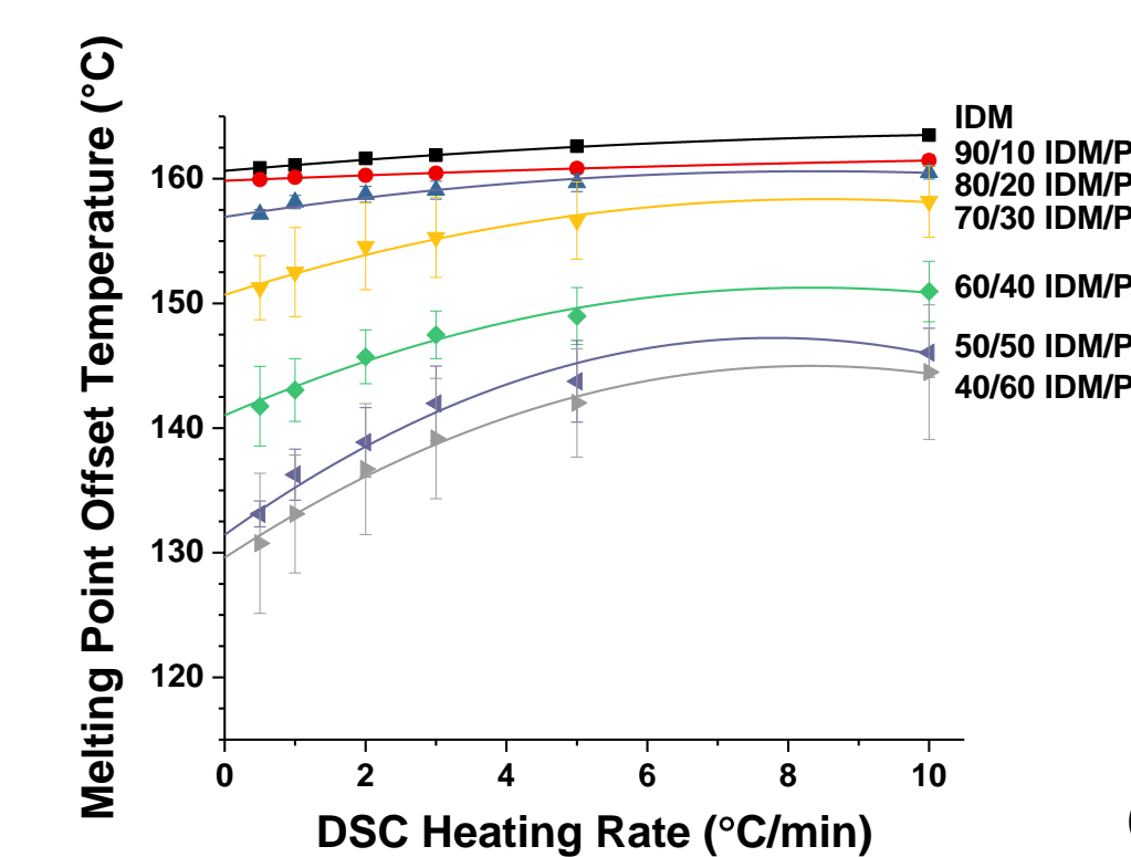
Figure 2. (a) Melting point depression is illustrated through DSC heat flow traces of various drug-polymer mixtures. (b) Melting point offset temperature is non-linear with respect to heating rate. (c) The interaction parameter \chi can be extracted by linear regression analysis.
