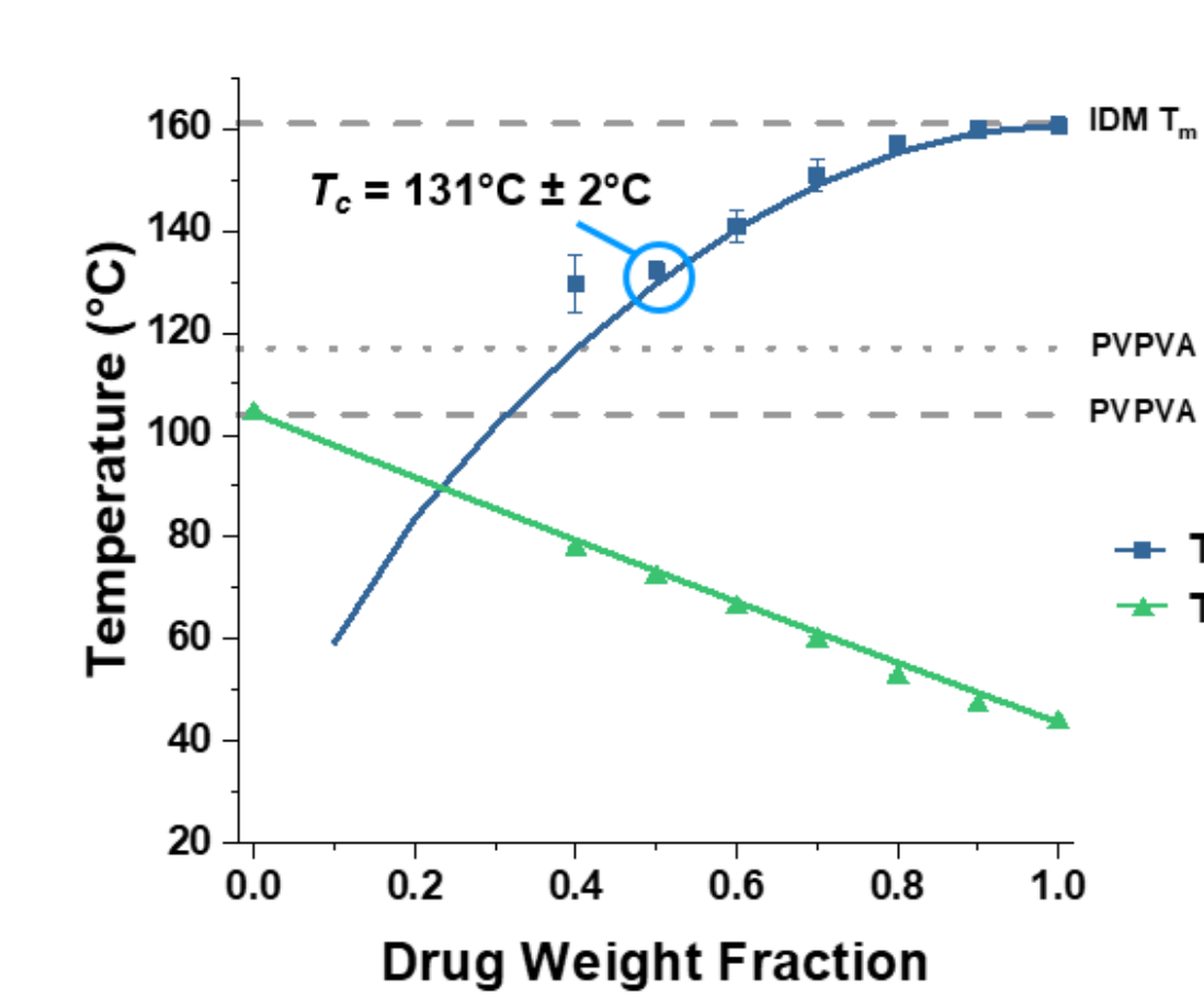
Figure 3. Indomethacin-PVPVA temperature-composition phase diagram, identifying the solubility line and glass transition temperature across the composition range.
