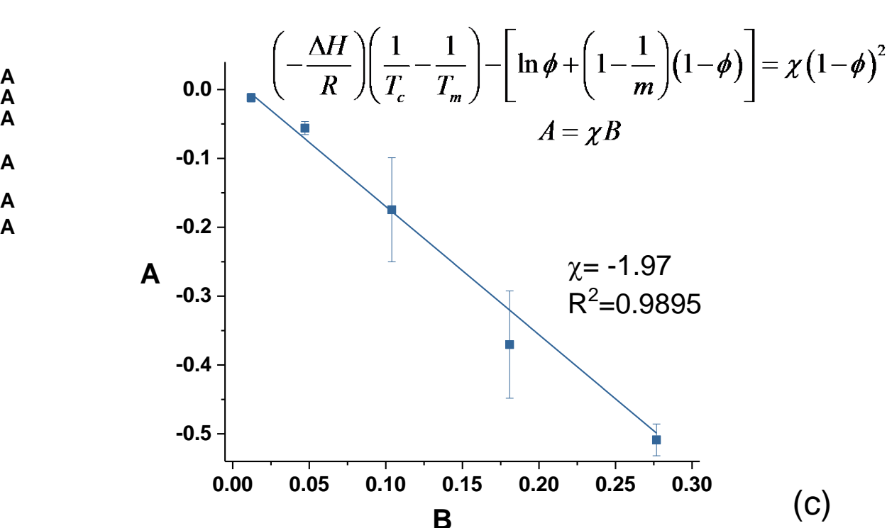
Figure 2. (a) Melting point depression is illustrated through DSC heat flow traces of various drug-polymer mixtures. (b) Melting point offset temperature is non-linear with respect to heating rate. (c) The interaction parameter \chi can be extracted by linear regression analysis.
