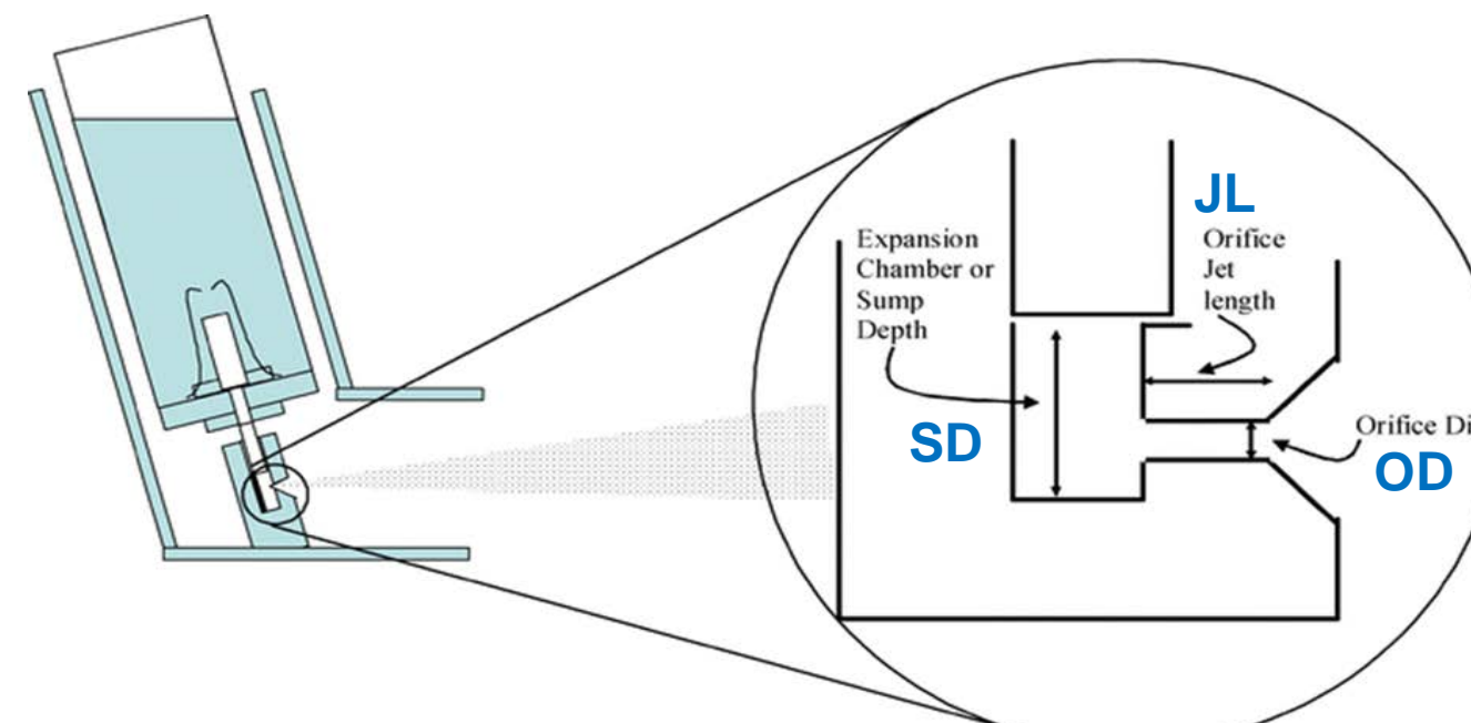
Figure 3. Design of MDI actuator parameters. 7
