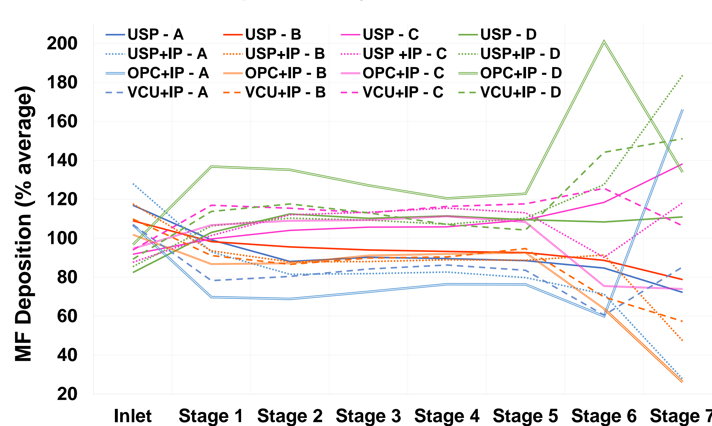
Figure 5. MF deposition (% average) on NGI stages by actuator variant (A, B, C, D) and APSD testing condition from all formulations. The % average for each APSD testing condition (e.g. USP+IP) = (mean MF deposition of each NGI stage by actuator) / (mean MF deposition of that NGI stage for all actuators) x 100%. USP: APSD testing using USP induction port and compendial method as described in USP <601>; 8 USP+IP / OPC+IP / VCU+IP: APSD testing using of IP with USP induction port or M-T model.
