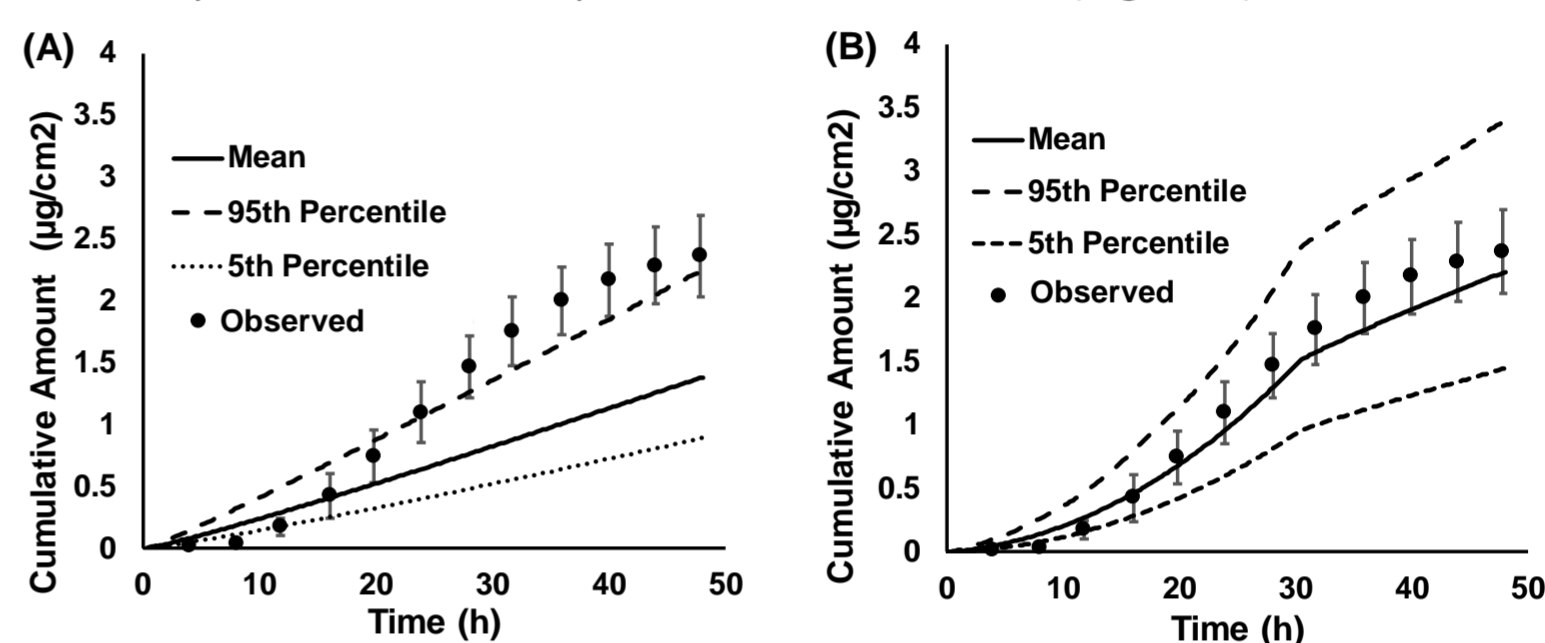
Figure 1. Mean cumulative permeation of Acyclovir following application of 15 mg/cm 2 of Zovirax® Cream, 5% (A) with constant stratum corneum lipid: vehicle partition coefficient and (B) with time-dependent stratum corneum lipid: vehicle partition coefficient considering the effect of propylene glycol on acyclovir skin permeation. Black circles with error bars (Mean ± SE, n= 6 donors with 4-7 replicates per donor) represent the observed data reported by Shin et al. 4
